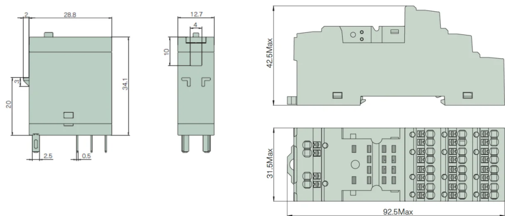
SOCKET GS 4C-PU Dimension Drawing
