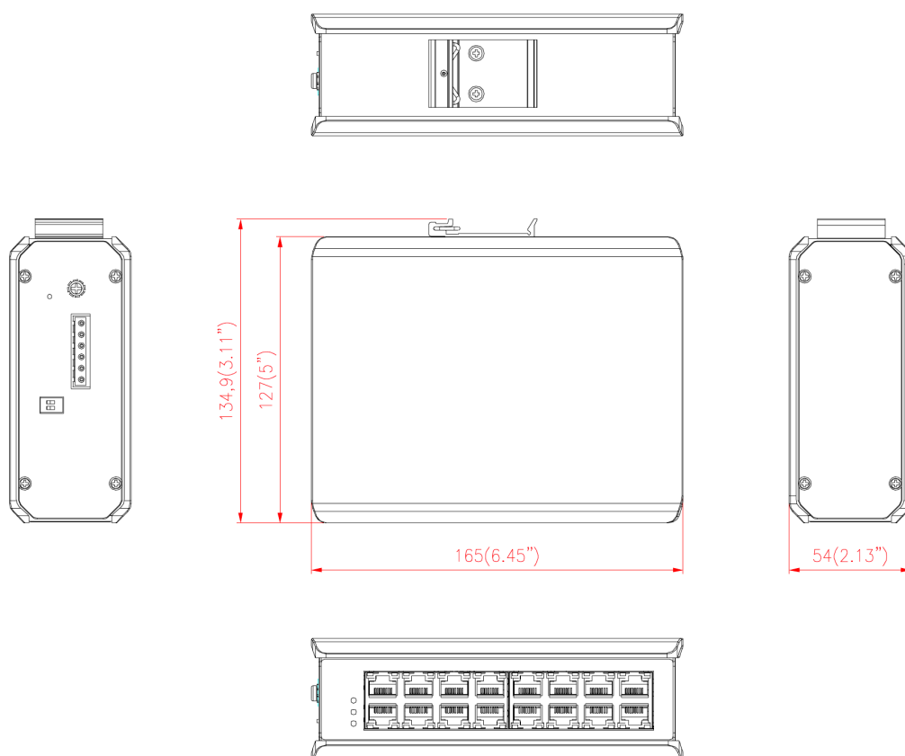
Dimension Drawing SWITCH 2016GT
